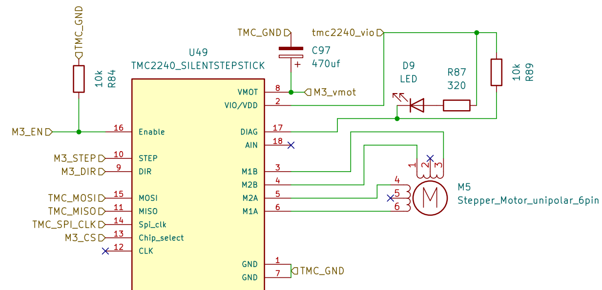
M3_control with TMC2240/TMC5160
