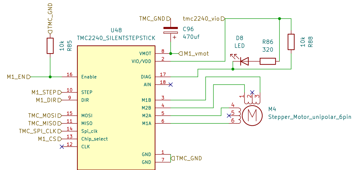
M1_control with TMC2240/TMC5160
