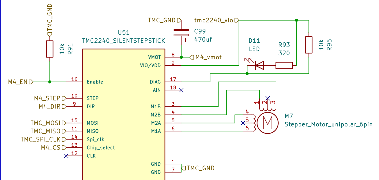
M4_control with TMC2240/TMC5160
