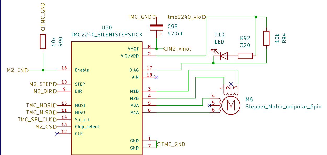
M2_control with TMC2240/TMC5160
